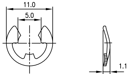
C-RING THICKNESS: 0.6mm (PACKAGED IN PE BAG SEPARATED)
